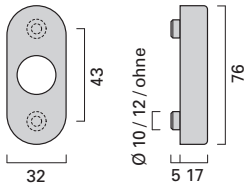
Fenster-Rosette F Window-Rose F
